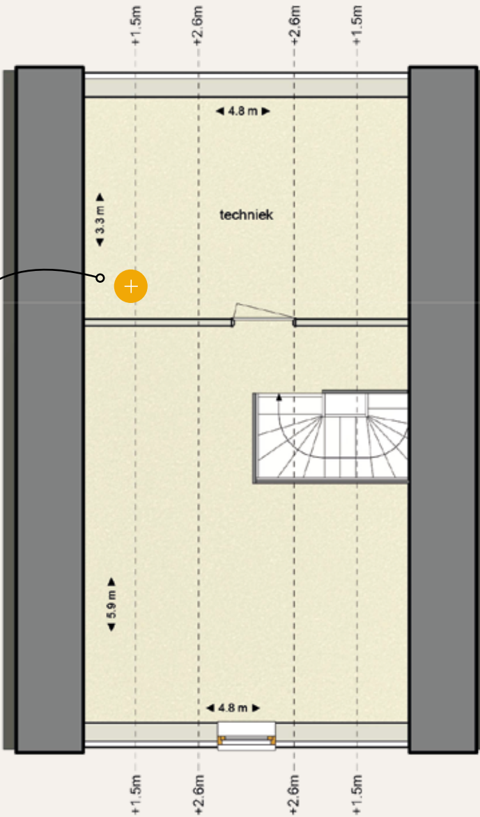
Zolder
